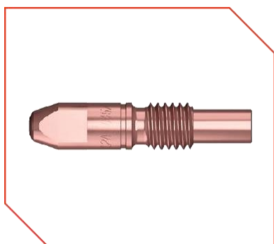
XP8 CONTACT TIP AL WIRE 1.0- 1.2MM
